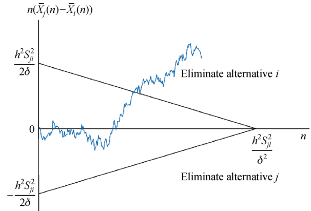
Fig. 1 Triangular region for the \mathcal{KN} procedures.
